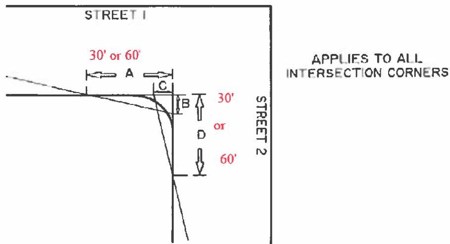
TYPICAL INTERSECTION CORNER
