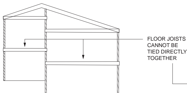
SECTION VIEW
