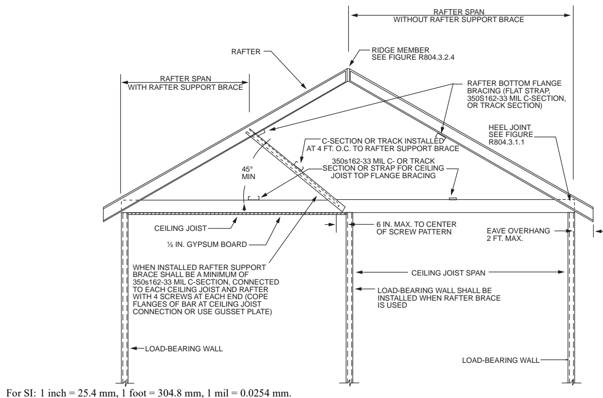
FIGURE R804.3 COLD-FORMED STEEL ROOF CONSTRUCTION
