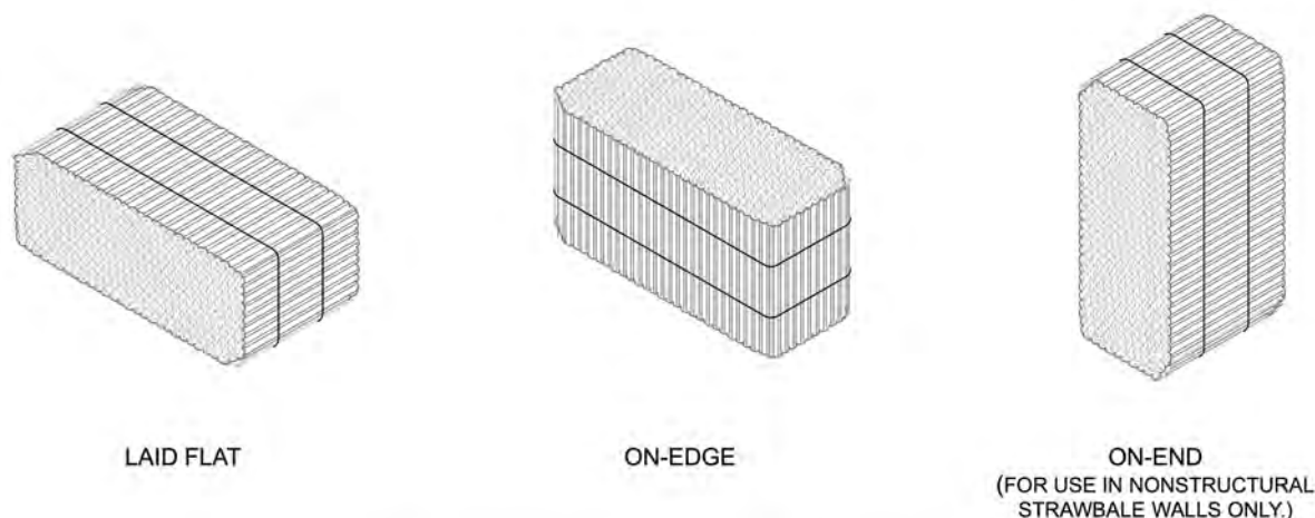
FIGURE AS101.1 TYPICAL STRAWBALE WALL SYSTEMS
