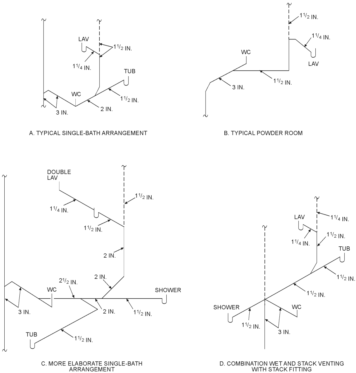
FIGURE N1 TYPICAL SINGLE-BATH WET-VENT ARRANGEMENTS
